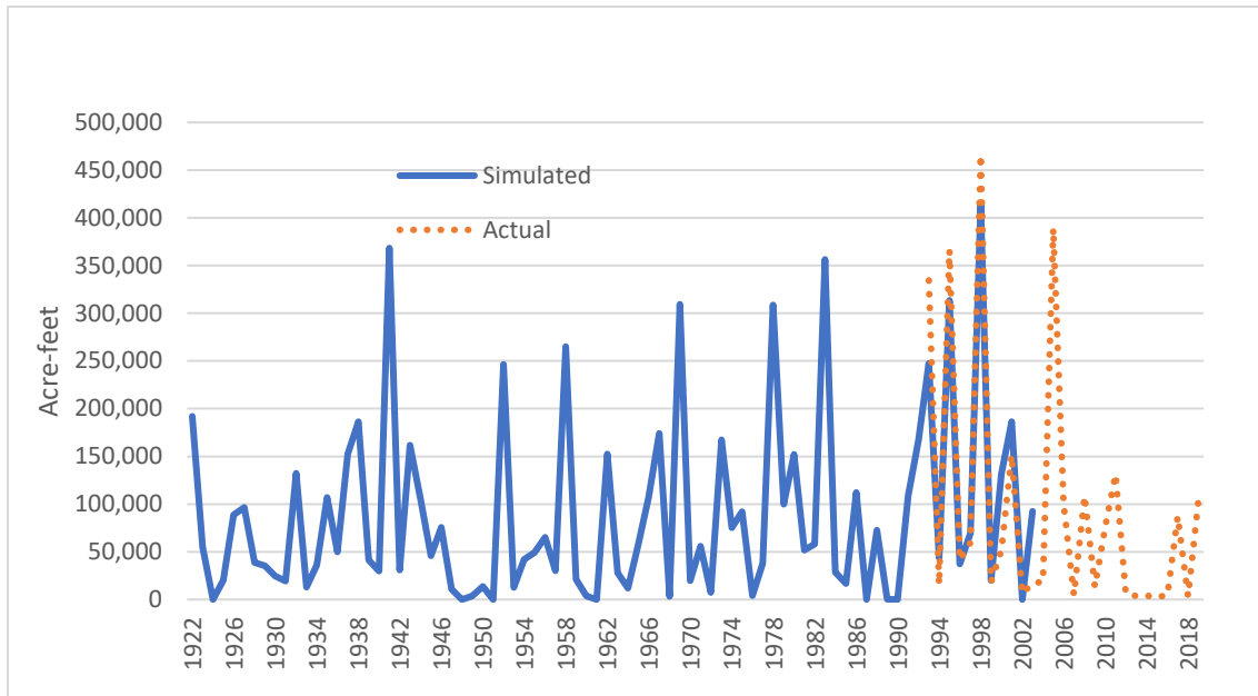
Figure E 3: Cachuma Reservoir Inflows
