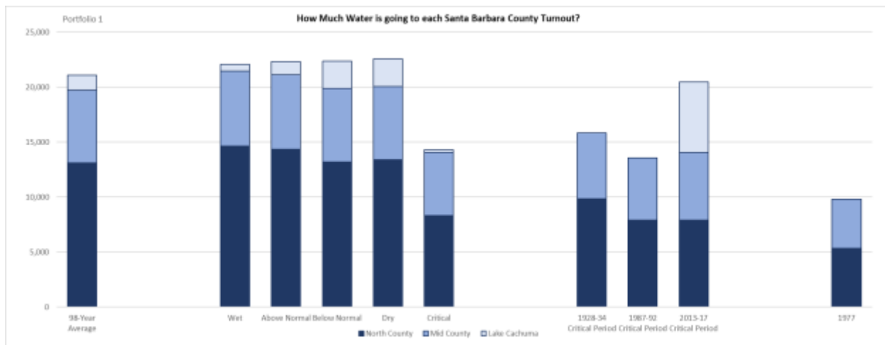
Figure 9-3 SWP Water Supply Deliveries to CCWA by Turnout Group
