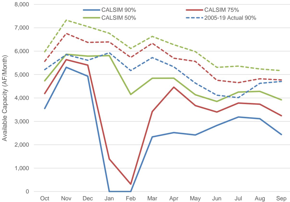
Figure 6-4 Coastal Aqueduct Polonio Pass Pumping Plant Capacity Availability
