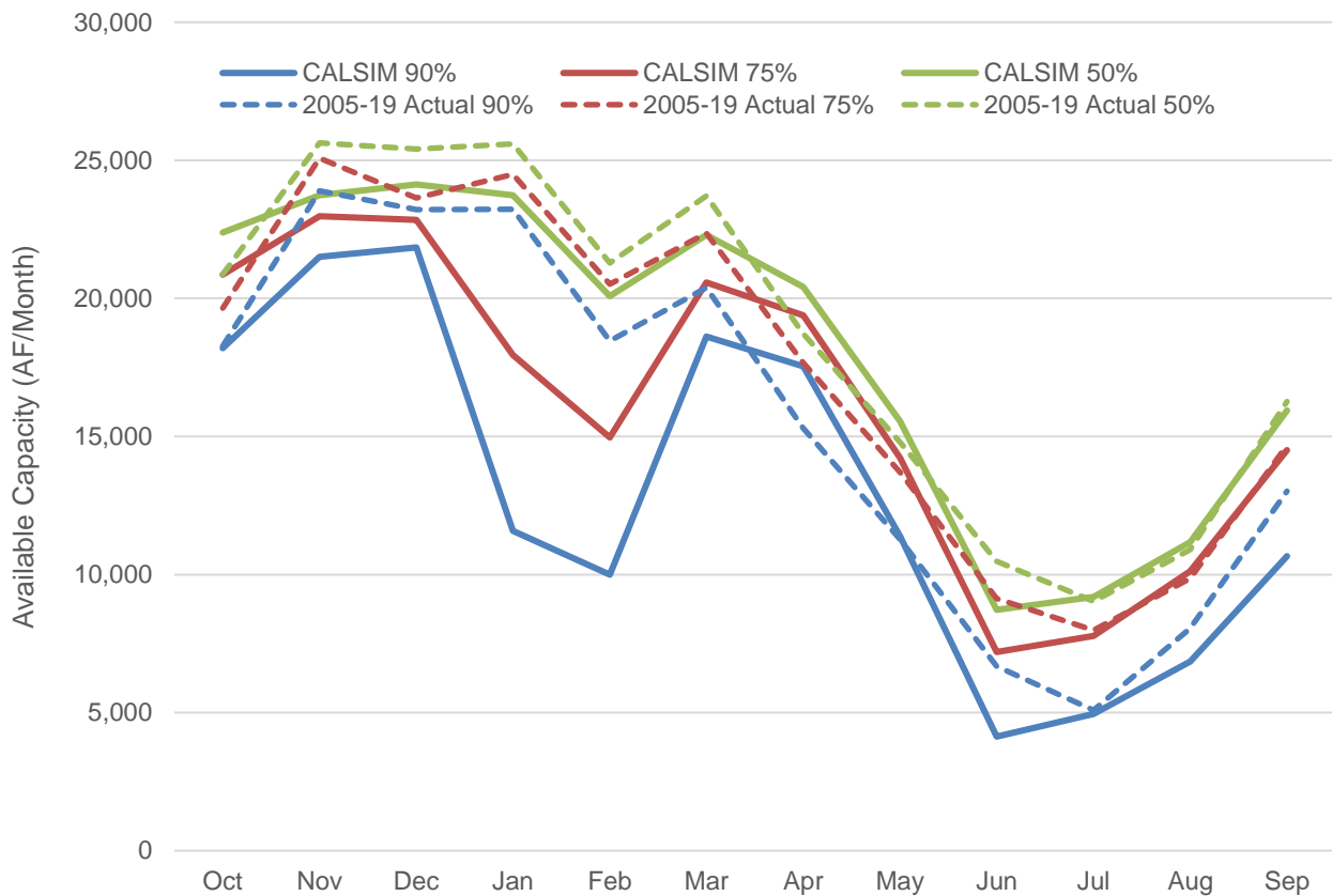
Figure 6-3 Coastal Aqueduct Badger Hill Pumping Plant Capacity Availability
