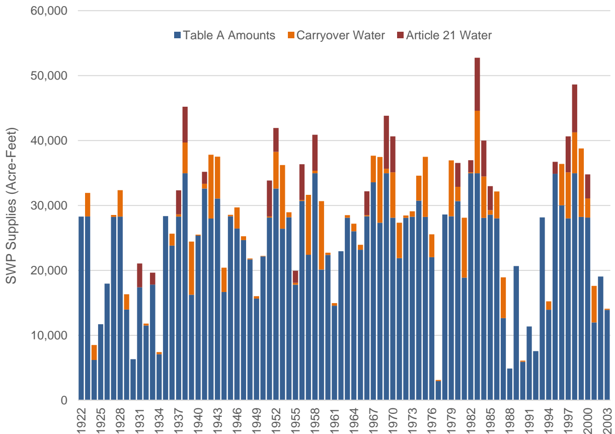
Figure 7-1 Santa Barbara County – SWP Available Supply Present Level
