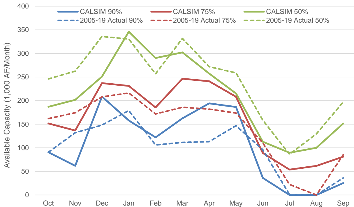
Figure 6-1 California Aqueduct Reach 7 (Check 21) Capacity Availability
