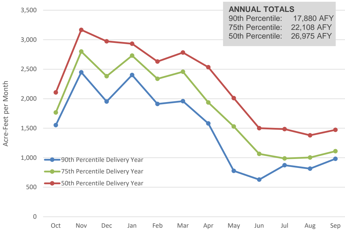
Figure 6-6 Reach 34 Historic (1998-2020) Capacity Availability
