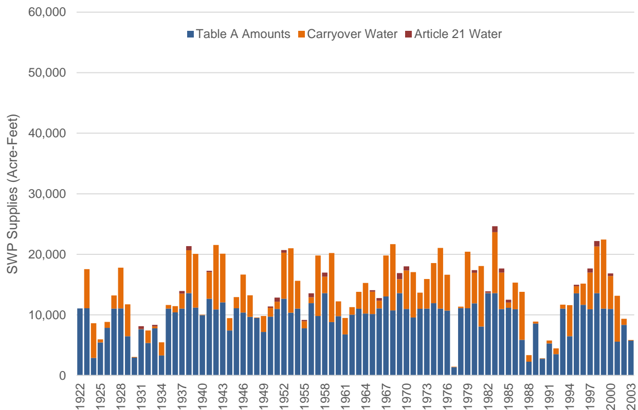
Figure 7-2 San Luis Obispo County -- SWP Available Supply Present Level -
